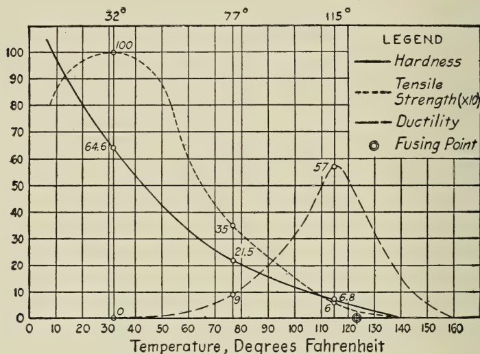
FIG. 113.—Chart of Physical Characteristics of D-Grade California Asphalt.
